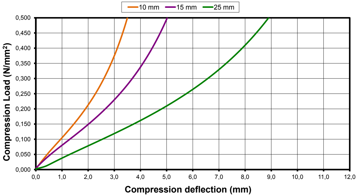
VS200 - Load Deflection Curve
