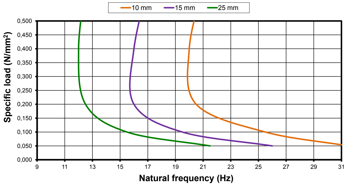
VS200 - Natural Frequency
