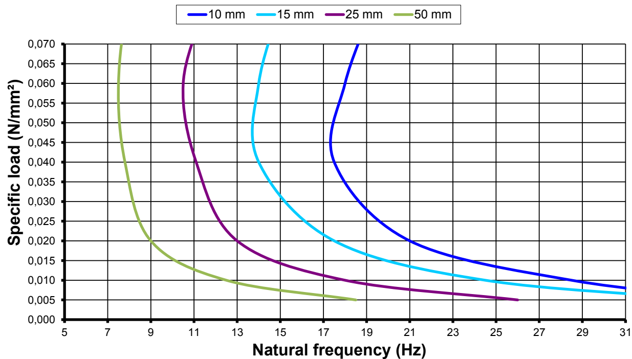
VS11 - Natural Frequency
