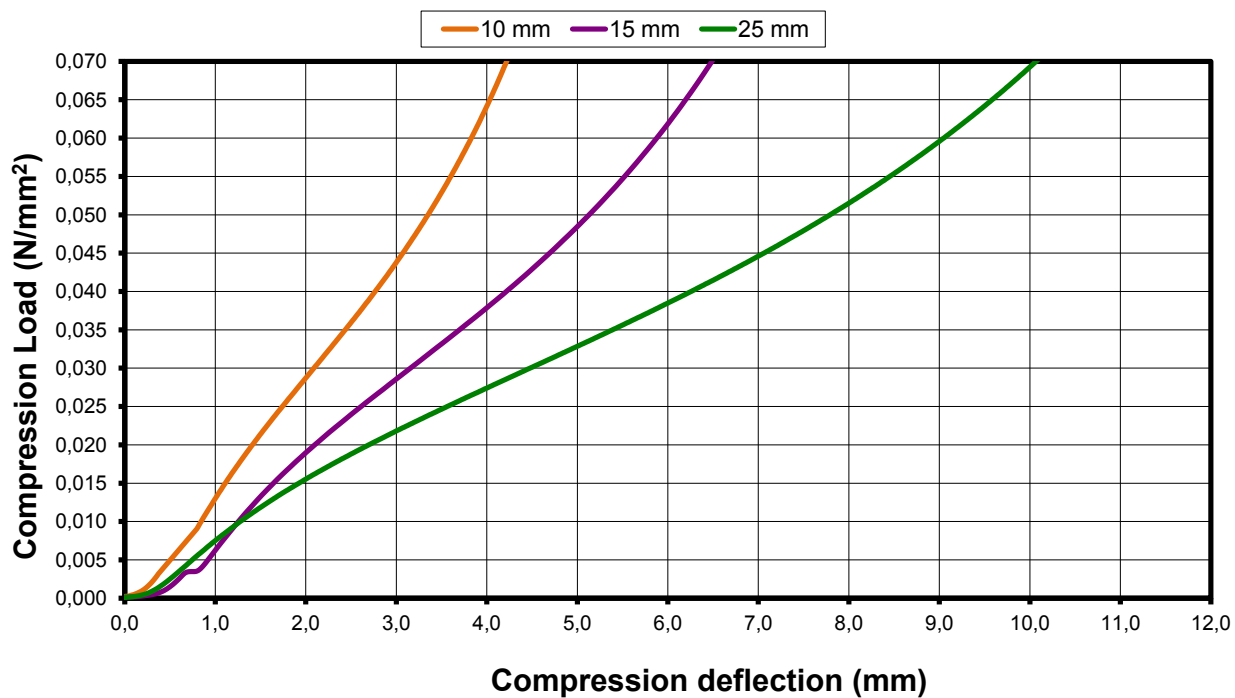
VS11 - Load Deflection Curve
