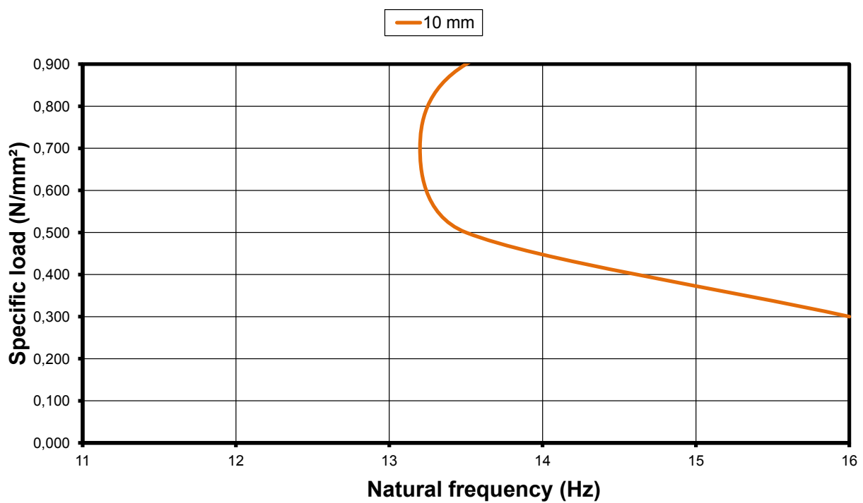
VM400 - Natural Frequency
