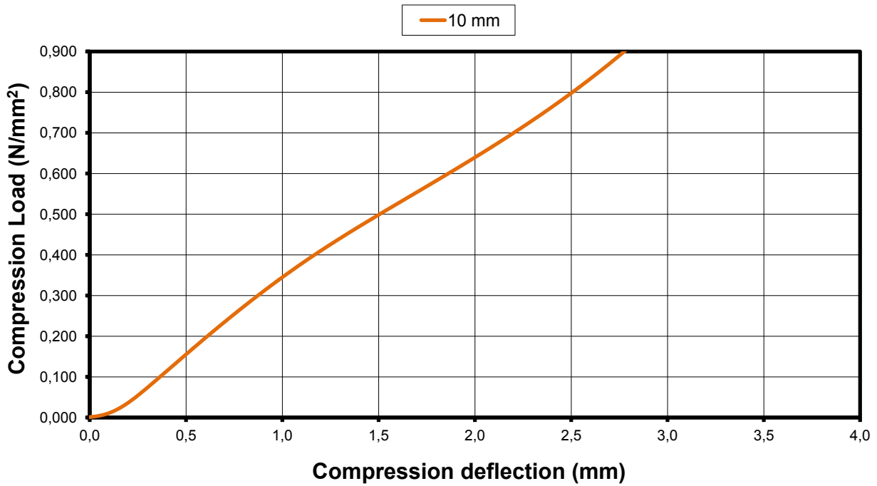
VM400 - Load Deflection Curve
